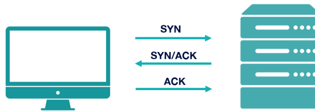
Three-Way Handshake
